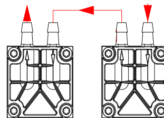
串联连接 Series Connection
