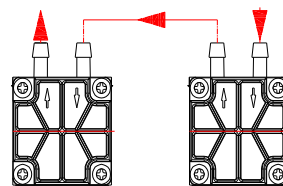
串联连接 Series Connection
